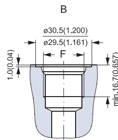
B: UNF main ports F: \frac{7}{8} - 14 UNF O-ring boss port
