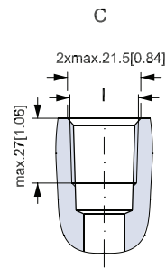
C: NPTF main I: \frac{1}{2} - 14 NPTF
