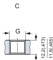
C: G drain port G: ISO 228/1 - G \frac{1}{4}
