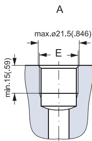
A: G main ports E: ISO 228/1 - G \frac{1}{2}
