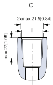
C: NPTF main ports I: ½ - 14 NPTF
