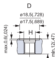
D: UNF drain port H: \frac{7}{16} - 20 UNF O-ring boss port
